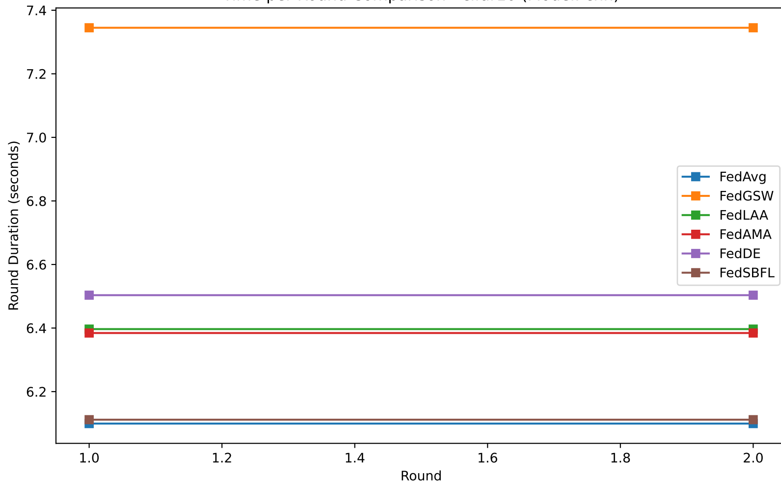
Time per Round Comparison - cifar10 (Model: cnn)
