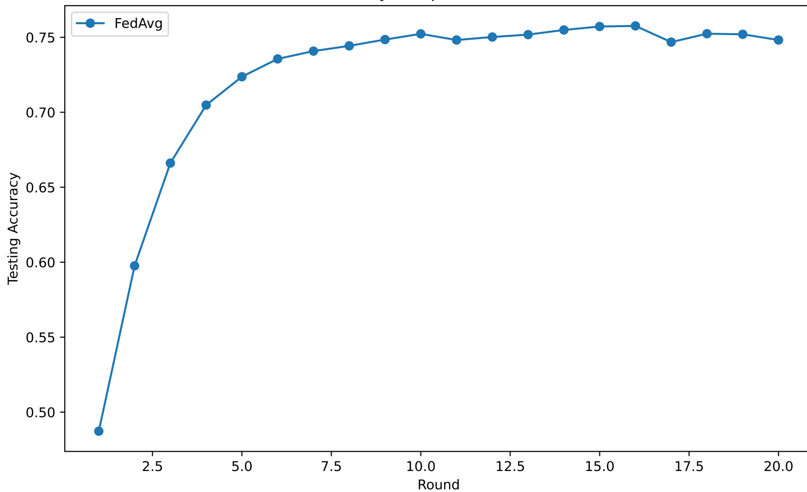
Accuracy Comparison - cifar10
