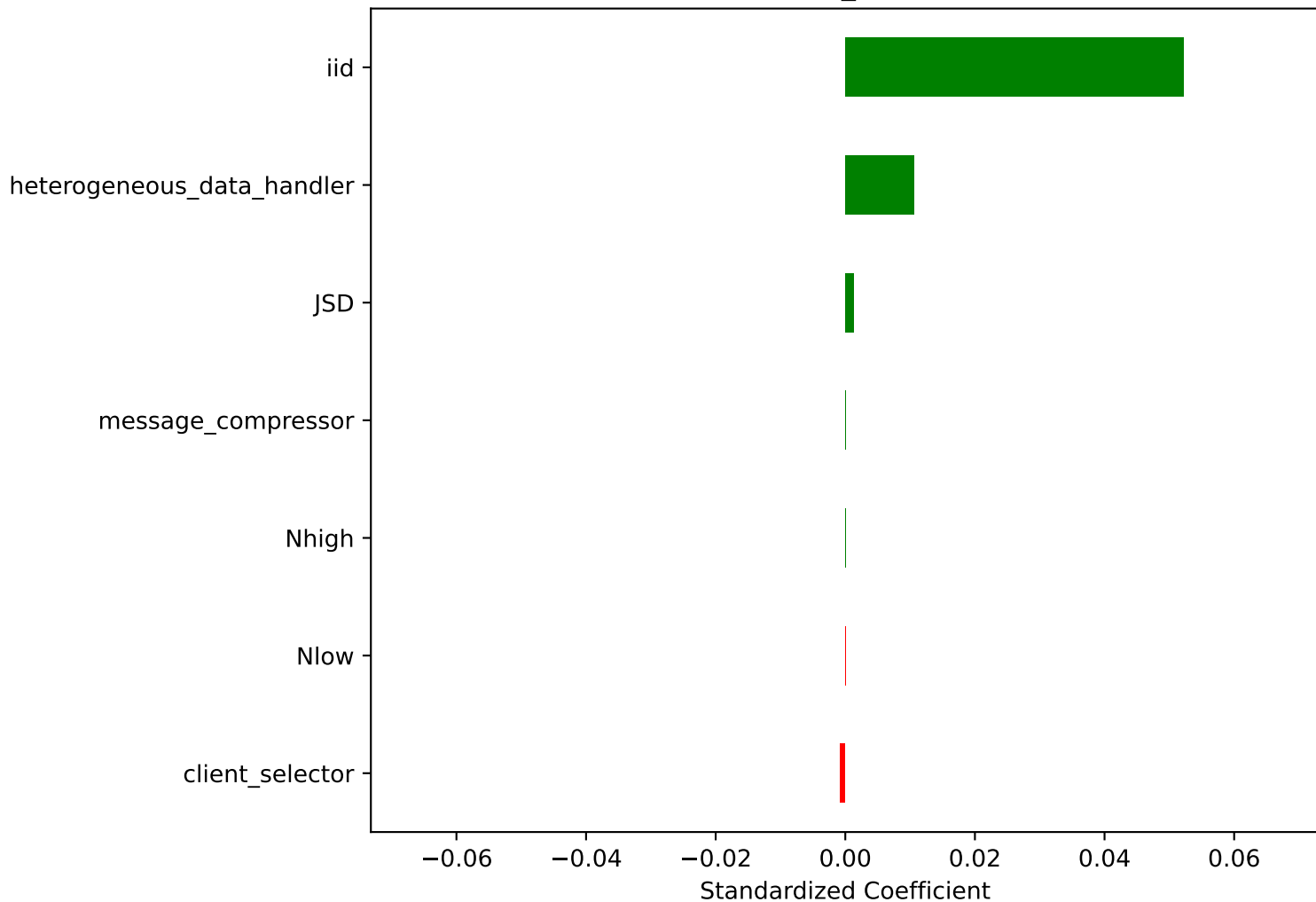
Linear Coefficients ( \Delta\text{ValF1} ) CNN 64k_CIFAR10
