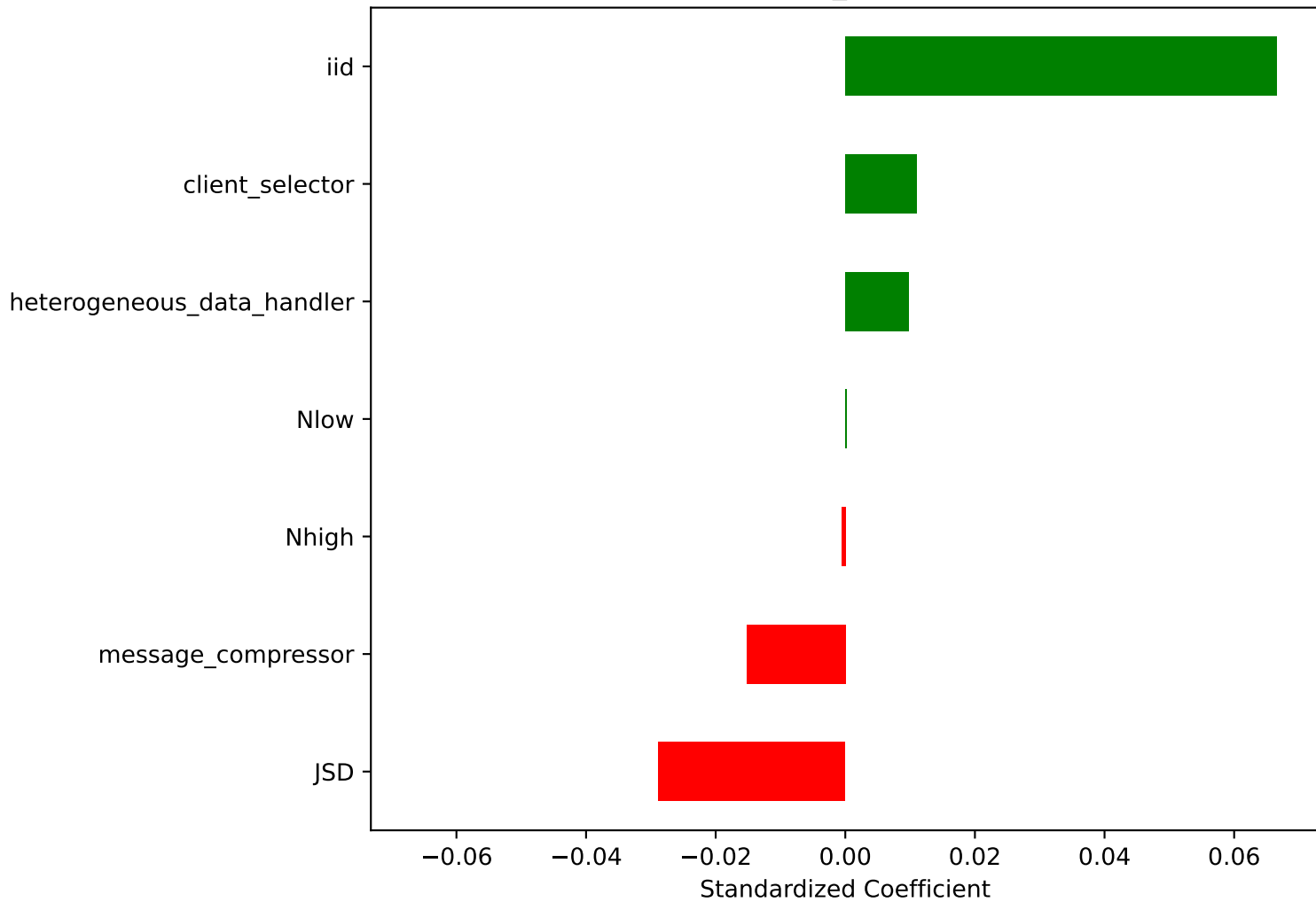
Linear Coefficients ( \Delta\text{ValF1} ) TextMLP_AGNEWS
