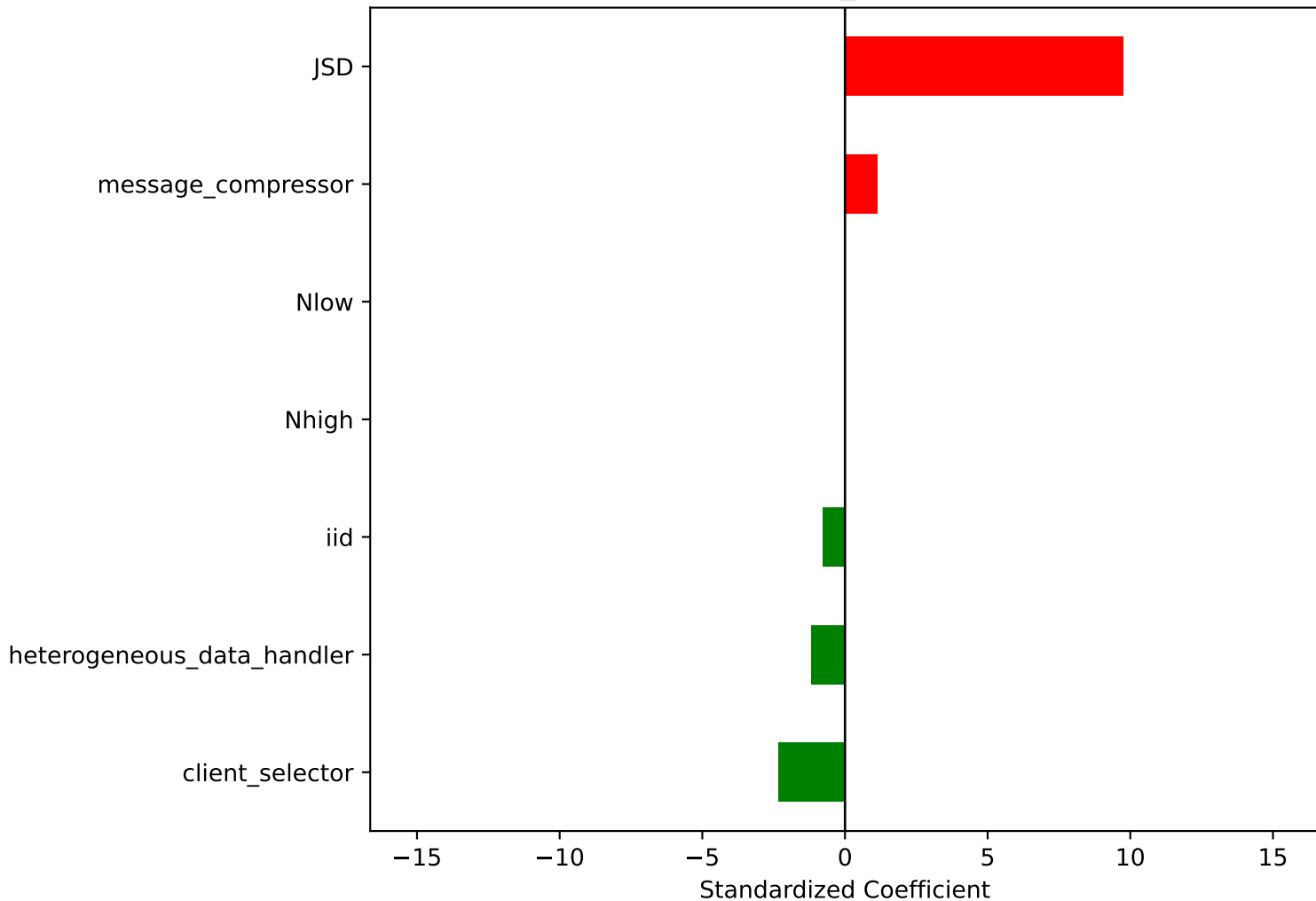
Linear Coefficients (Round Time) CNN 64k_CIFAR10
