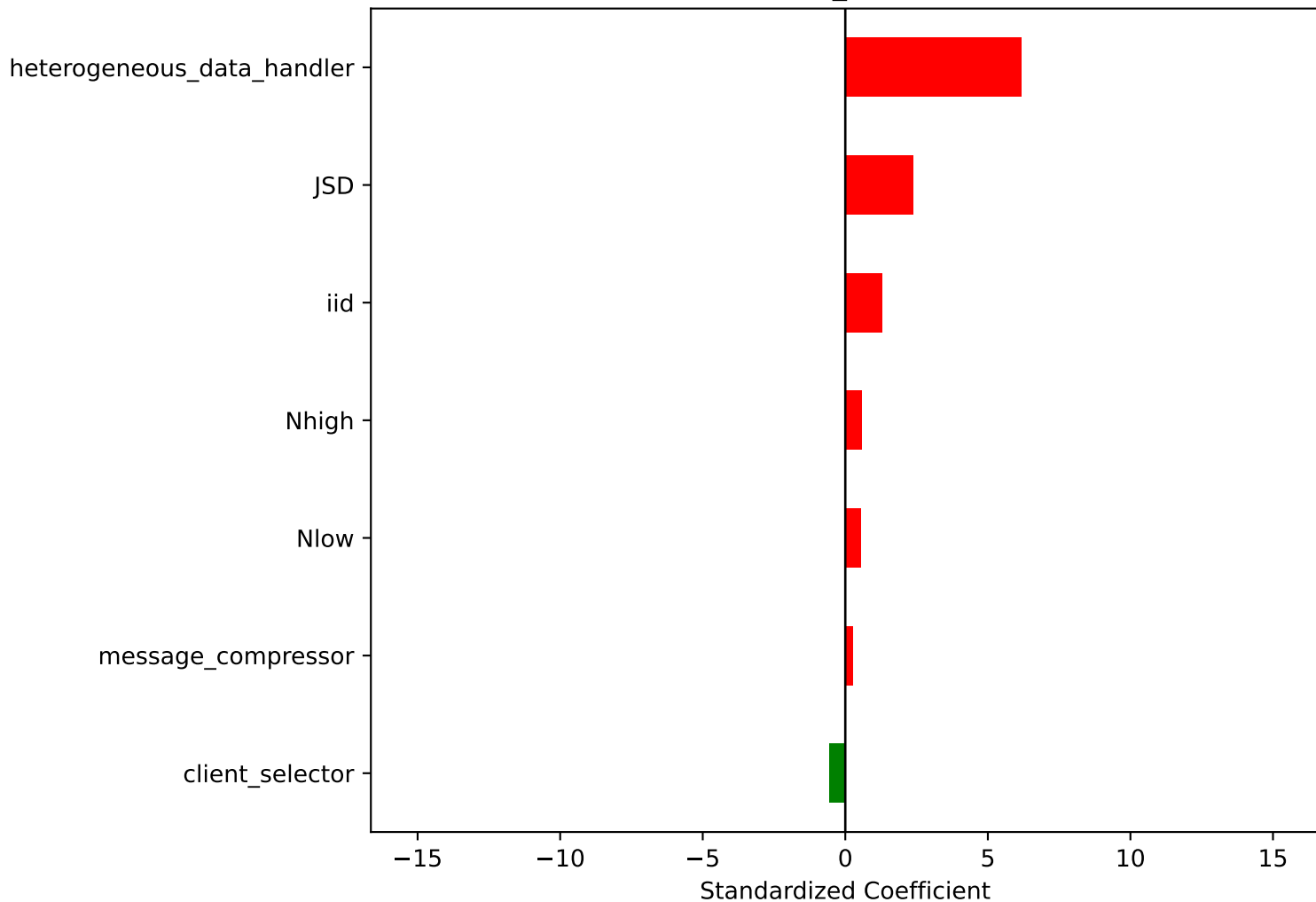
Linear Coefficients (Round Time) TextMLP_AGNEWS
