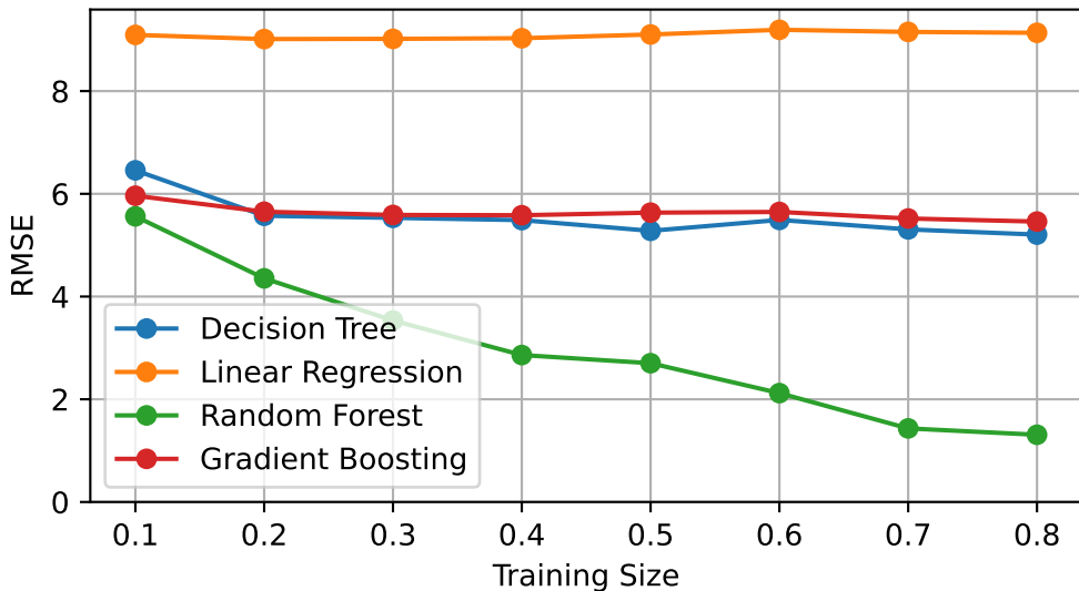
RMSE vs. Training Size for Different Regressors
