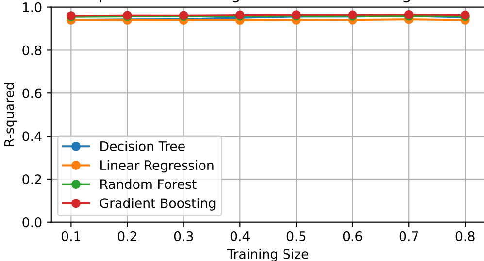
R-squared vs. Training Size for Different Regressors
