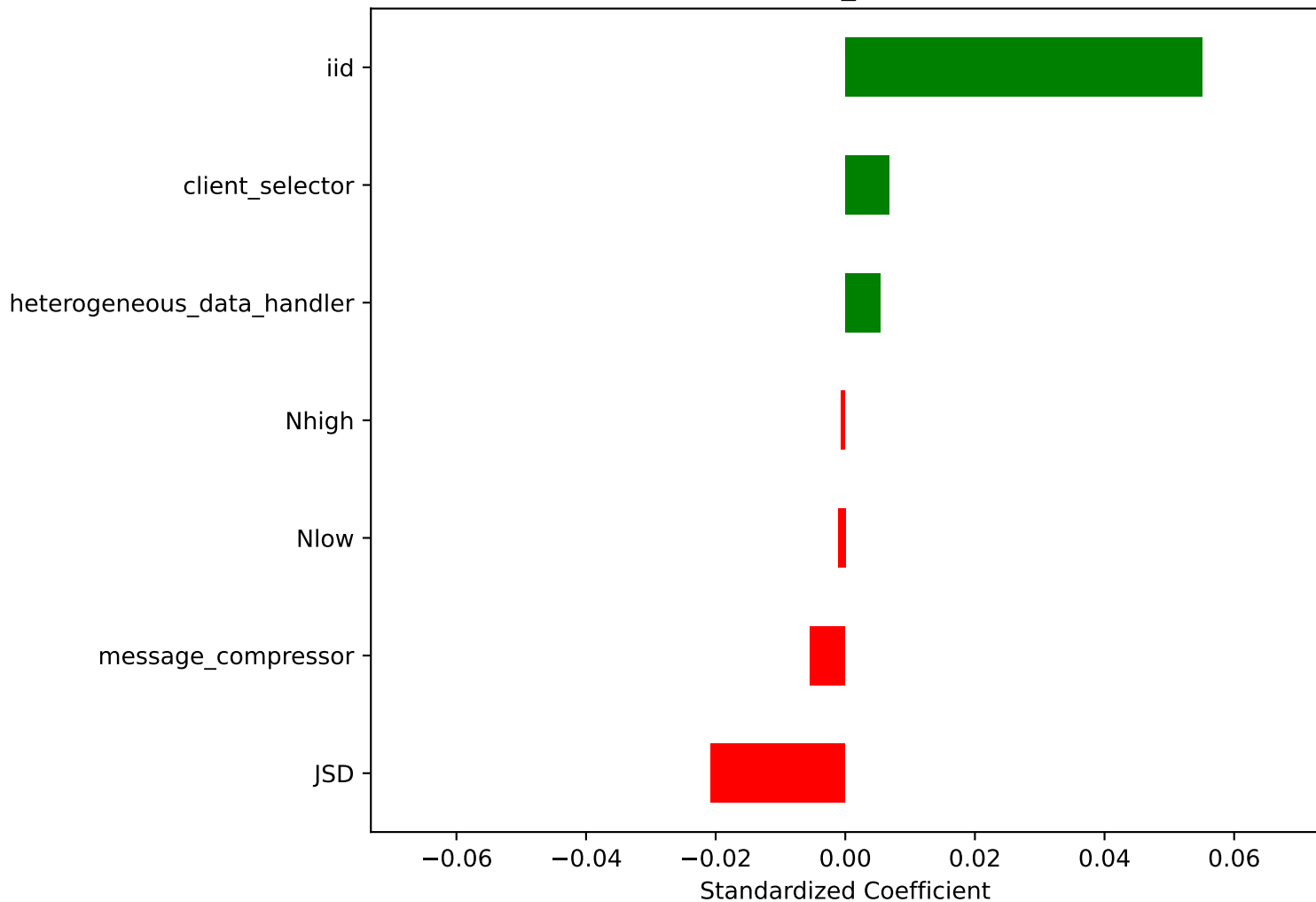
Linear Coefficients ( \Delta\text{ValF1} ) CNN 16k_CIFAR10
