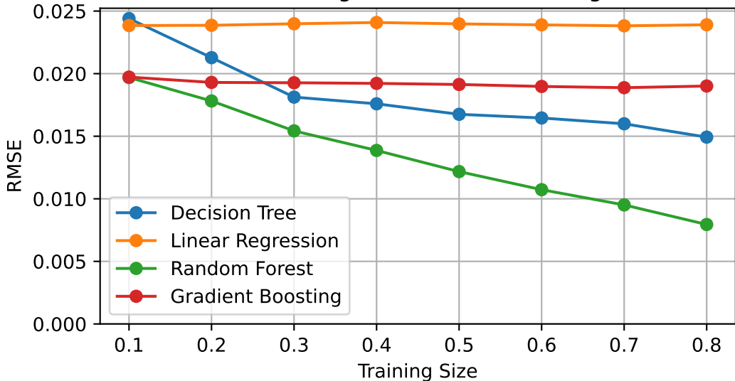
RMSE vs. Training Size for Different Regressors
