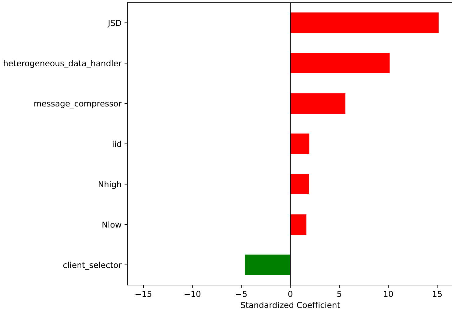
Linear Coefficients (Round Time) CNN 16k_CIFAR10
