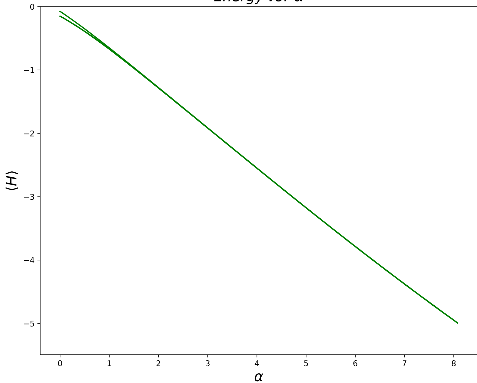
Energy vs. \alpha
