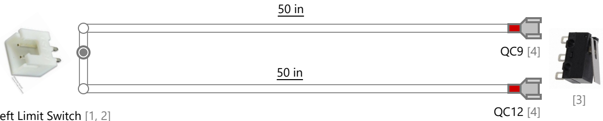
Z axis Left Limit Switch [1, 2]
