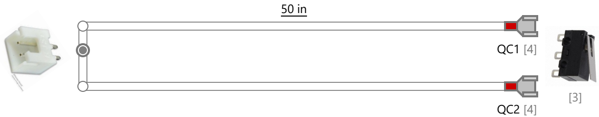
X axis Left Limit Switch [1, 2]
