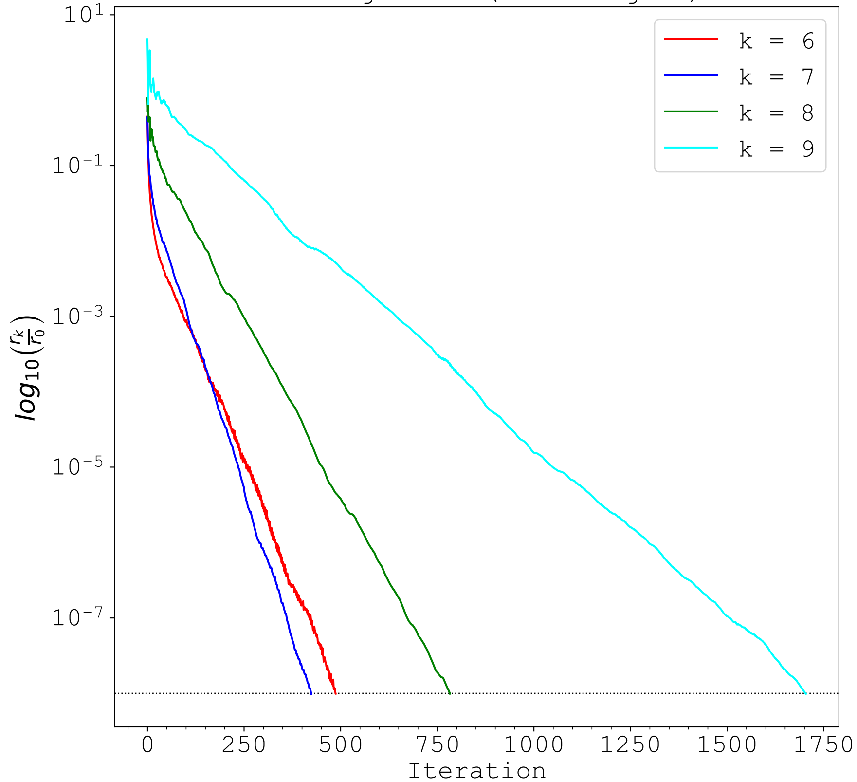
On-the-grid CG (no multigrid)
