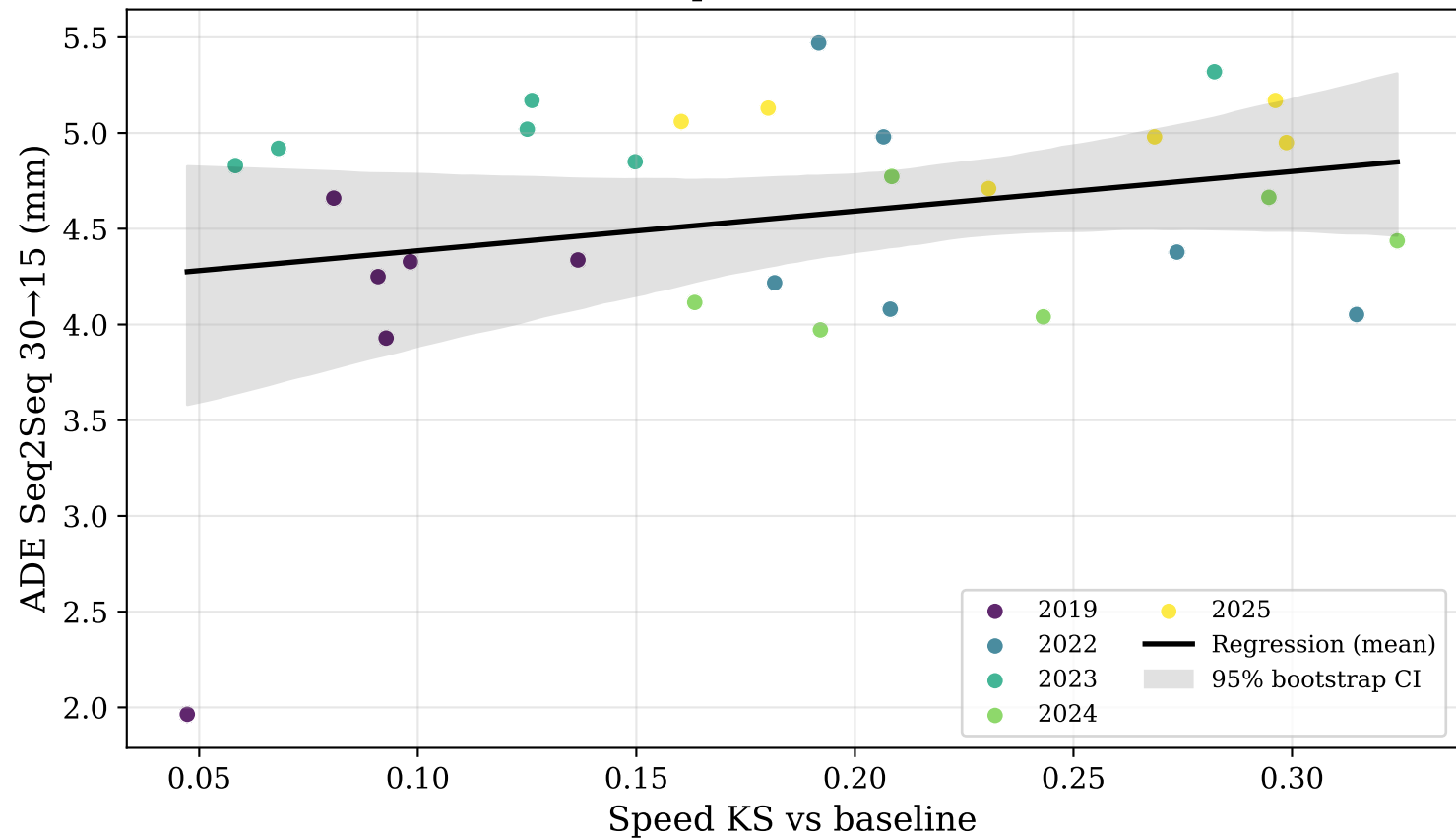
ADE vs Speed KS vs baseline
