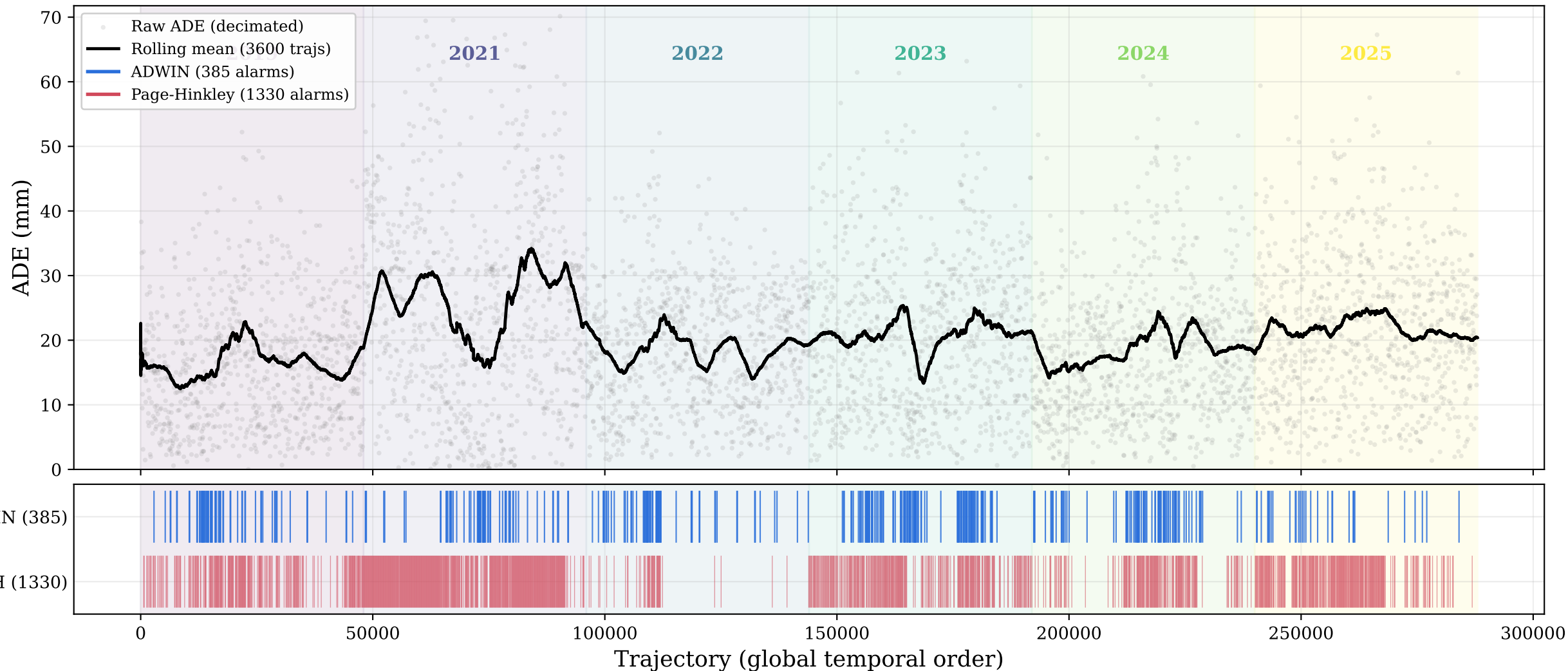
Online concept drift --- Kalman 30→15 ADE
