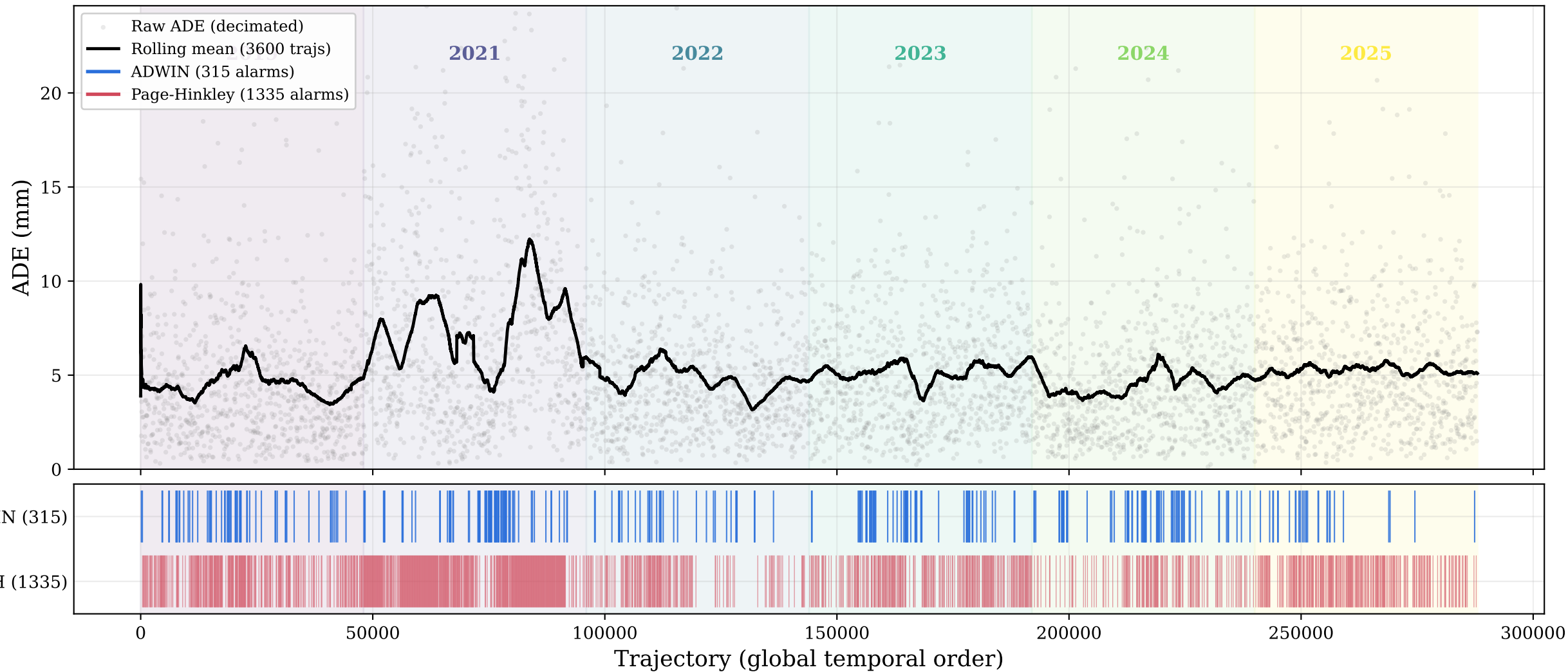
Online concept drift --- Seq2Seq 30→15 ADE
