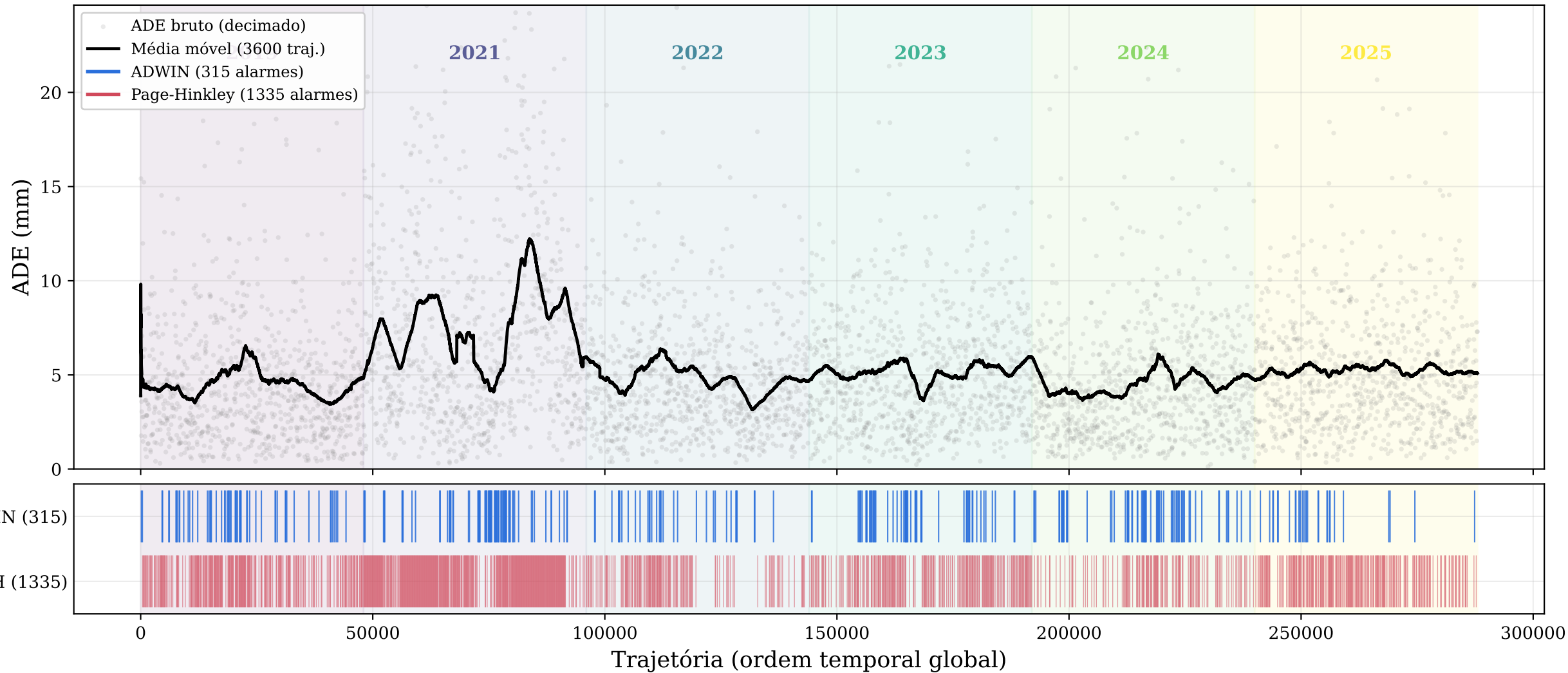
Concept drift online --- ADE Seq2Seq 30→15
