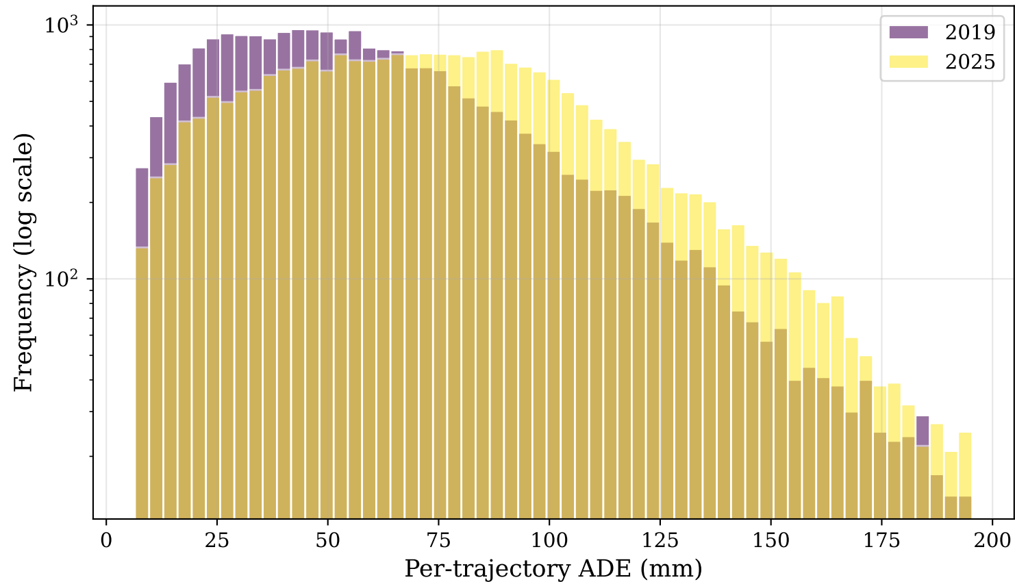
ADE distribution — Kalman 60→30
