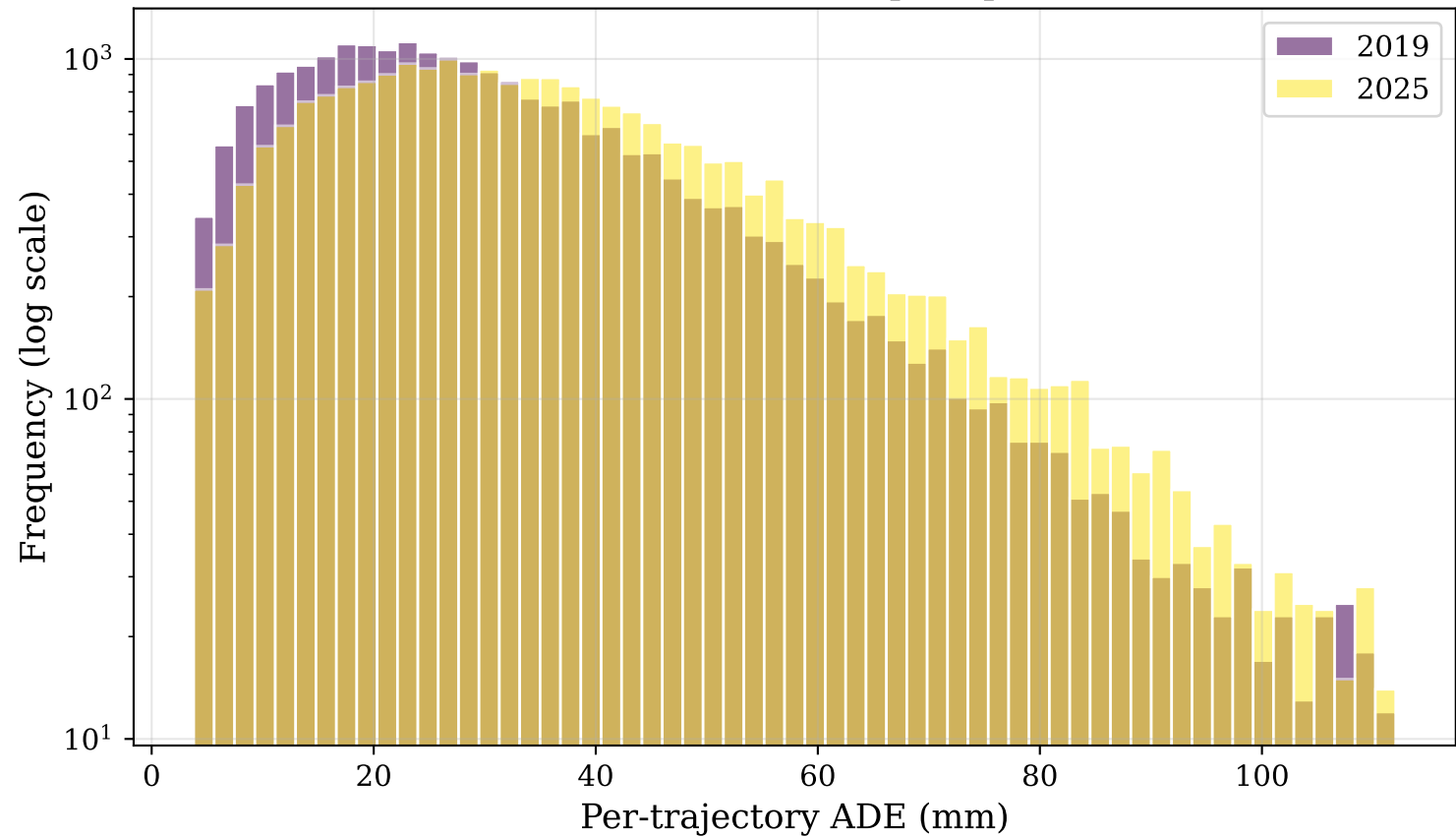
ADE distribution — Seq2Seq 60→30
