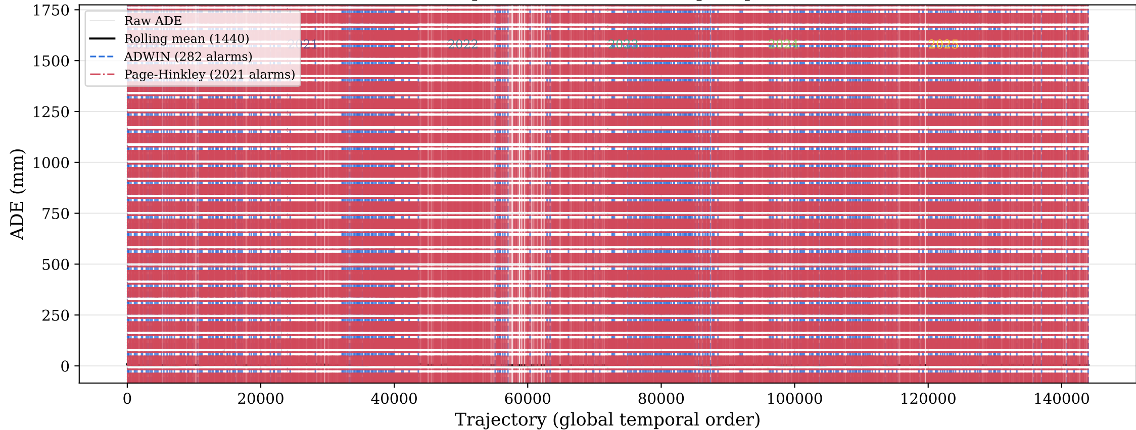
Online concept-drift detection — Seq2Seq 30→15 ADE
