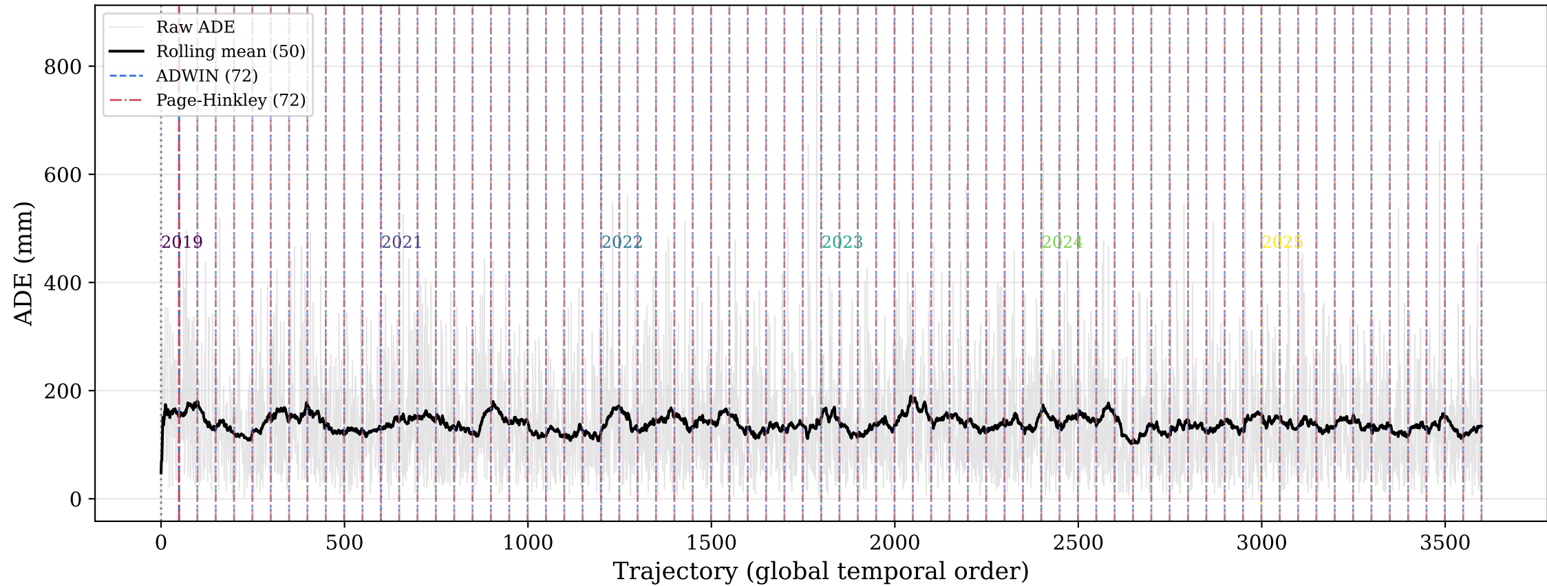
Online concept drift — Kalman 30→15
