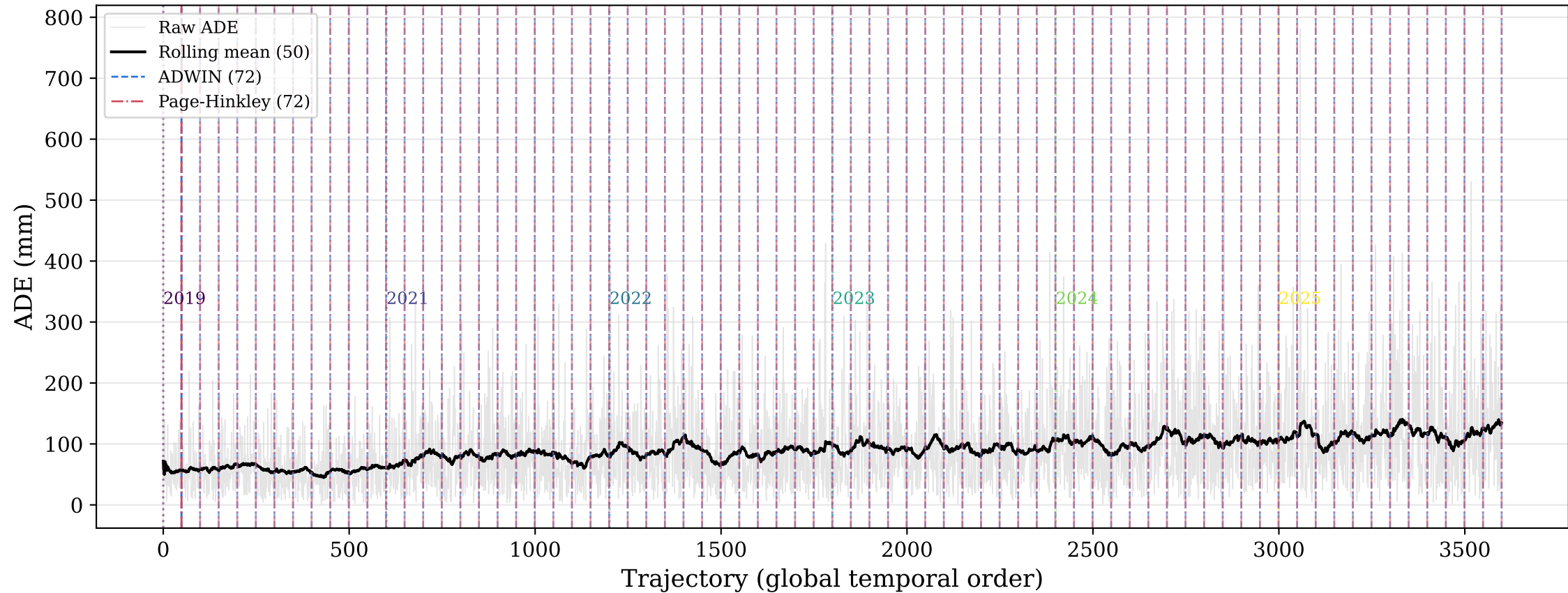
Online concept drift — Seq2Seq 30→15
