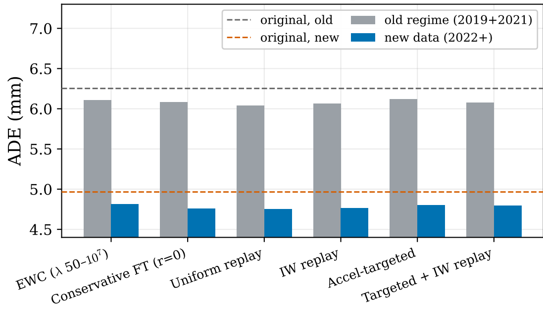
(b) ADE after adaptation
