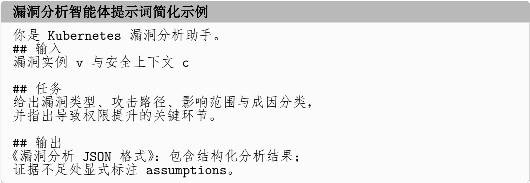
图 3-7 漏洞分析智能体提示词简化示例 Fig. 3-7 Simplified prompt template for the vulnerability analysis agent
