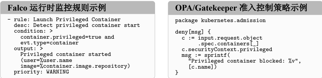
图 2-6 Falco 运行时监控规则与 OPA/Gatekeeper 准入控制策略示例 Fig. 2-6 Examples of a Falco Runtime Monitoring Rule and an OPA/Gatekeeper Admission Control Policy
