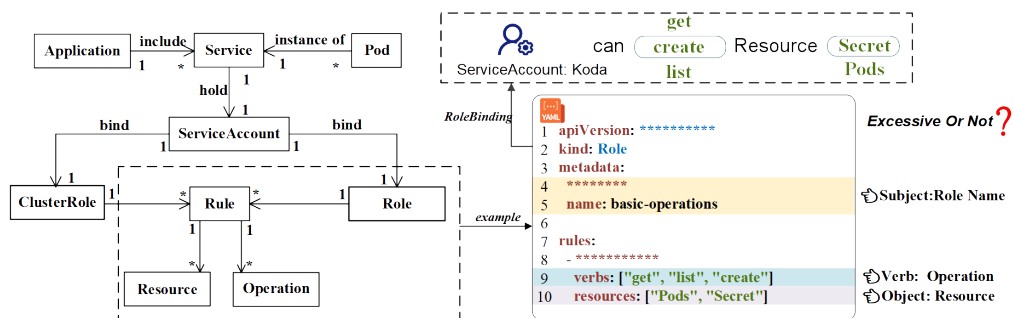
图 2-3: Kubernetes RBAC 权限配置 (YAML) 示意 [10]
