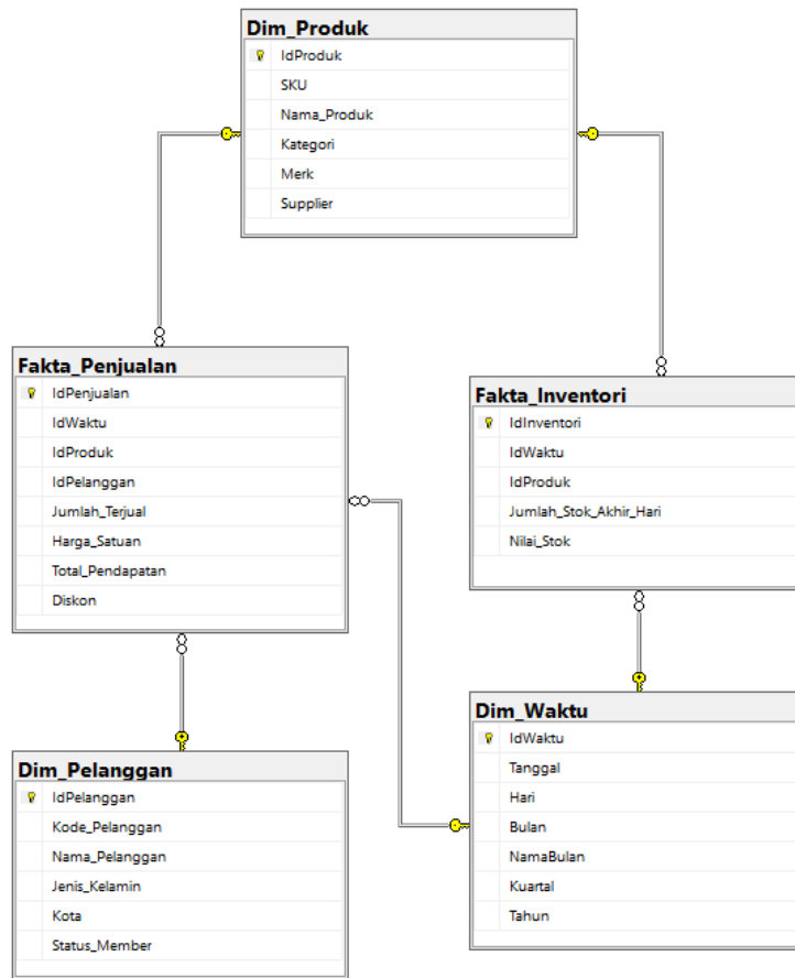
Gambar 1 Galaxy Schema
