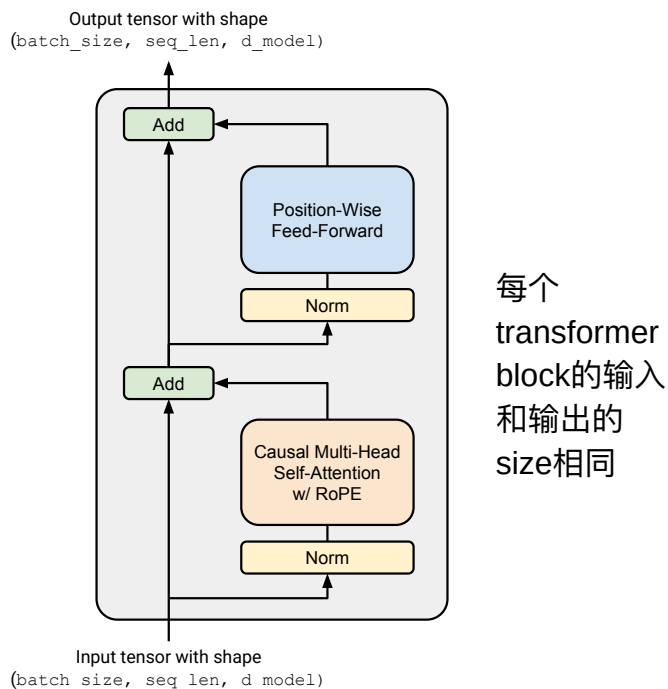
Figure 2: A pre-norm Transformer block.
