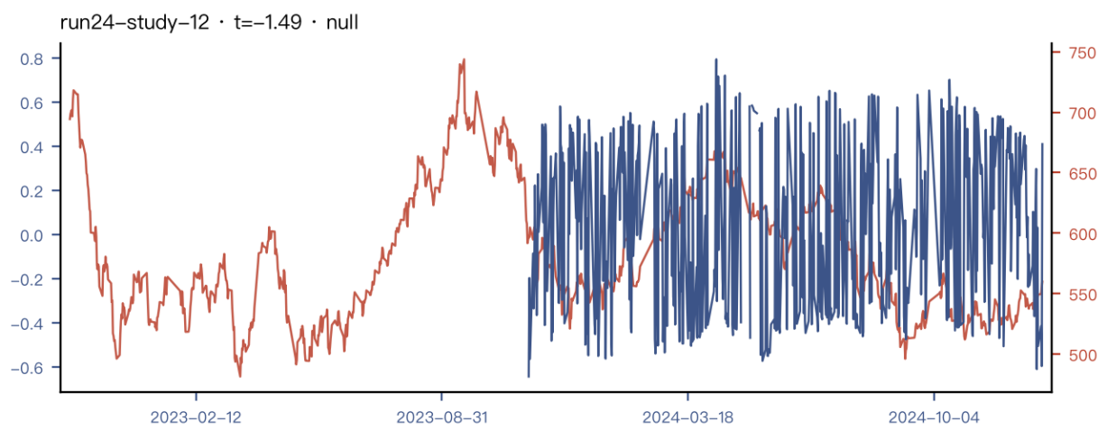
run24-study-12: pm_ceasefire_terminal_settlement_within_own_range_evt7d_resid_brent_1d_90d_pg。有定义 558/1040 点。
