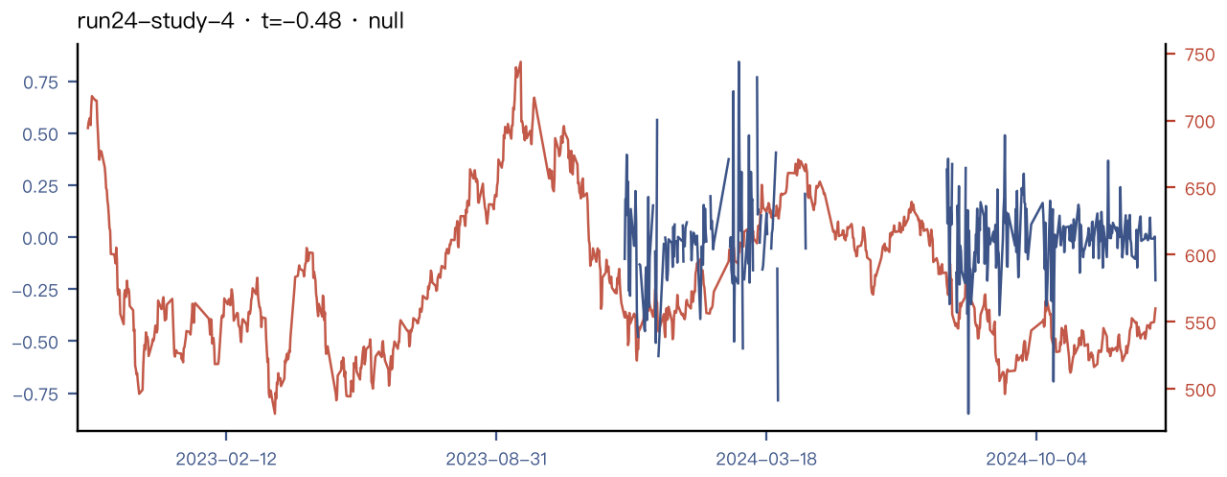
run24-study-4: pm_ceasefire_breakdown_disp_evt_resid_brent_3h_halves_90d_p。有定义 351/1040 点。
