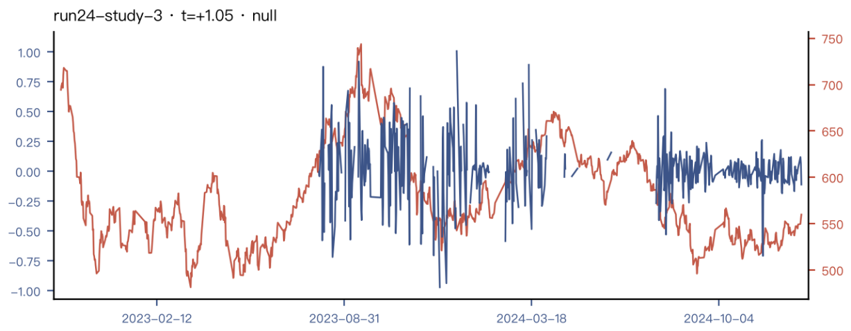
run24-study-3: pm_russia_escalation_hazard_same_phase_dod_revision_resid_brent_12h_90d_au。有定义 533/1040 点。
