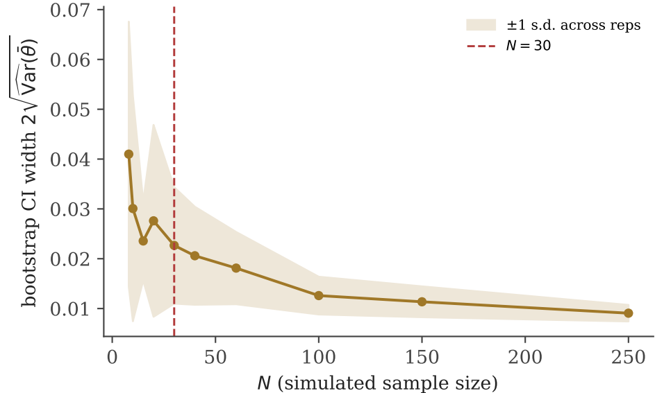
Bootstrap stability vs. N
