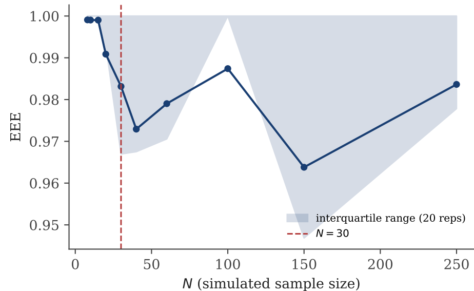
EEE vs. N
