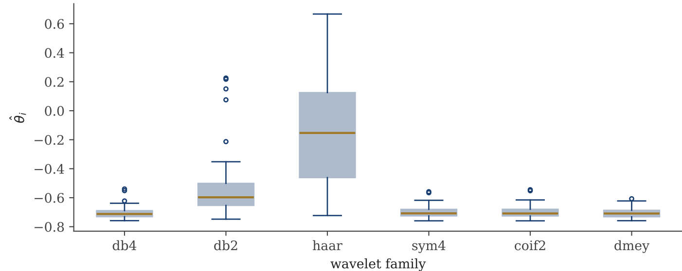
Sensitivity of \hat{\theta} to wavelet family (same 60 simulated signals)
