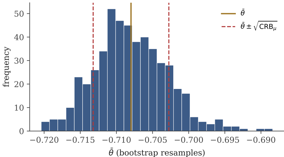
Bootstrap of \bar{\theta} vs. Cramér--Rao band (simulated EEE = 100.0%)
