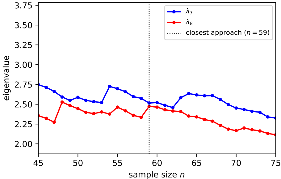
Avoided crossing, \lambda_7 - \lambda_8
