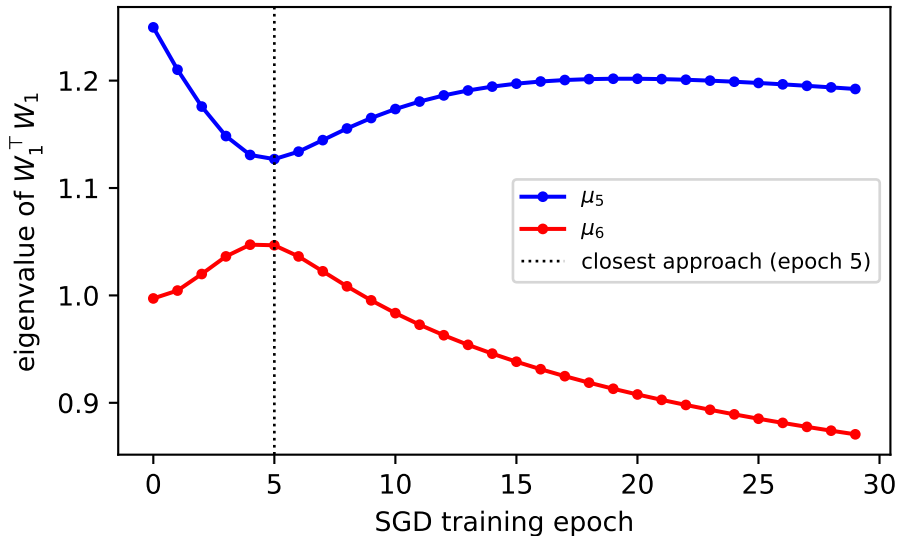
Classifier weight-matrix avoided crossing, \mu_5 - \mu_6 , seed 17, early training transient
