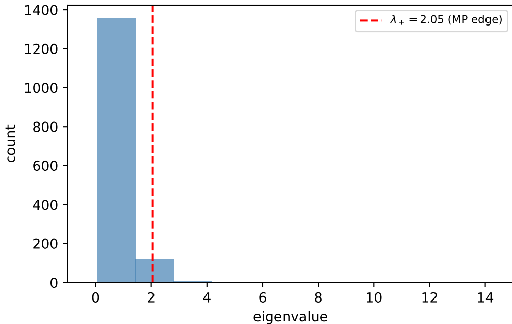
Raw correlation-matrix spectrum, single-cell TNBC (33/1500 eigenvalues exceed \lambda_+ , not all shown)
