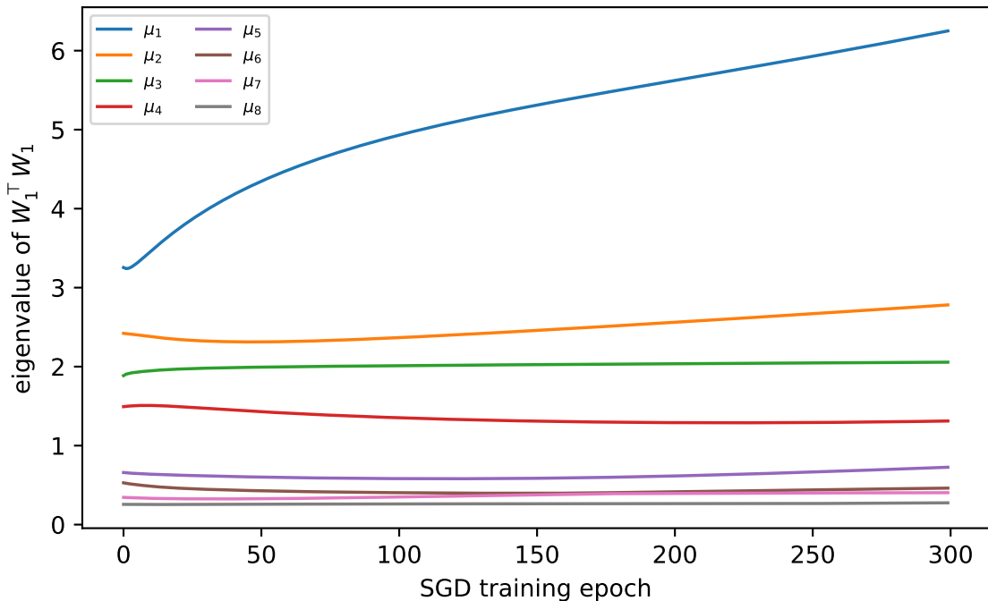
Classifier weight-matrix eigenvalue trajectories (seed 0, MLP(20 \rightarrow 8 \rightarrow 1), RMT-hub input genes)
