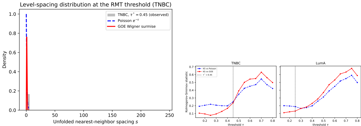
Figure 2: Left: unfolded nearest-neighbor spacing distribution for the TNBC network at \tau^* = 0.45 , against the Poisson and GOE (Wigner surmise) null curves. Right: Kolmogorov–Smirnov distance to each null curve as a function of threshold, for TNBC and LumA separately; the dotted line marks the selected \tau^* in each panel.
