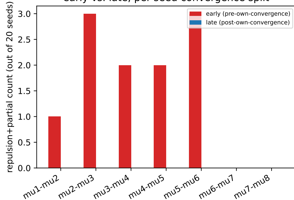
Longer-transient run (lr=0.01, 1500 epochs): early vs. late, per-seed convergence split
