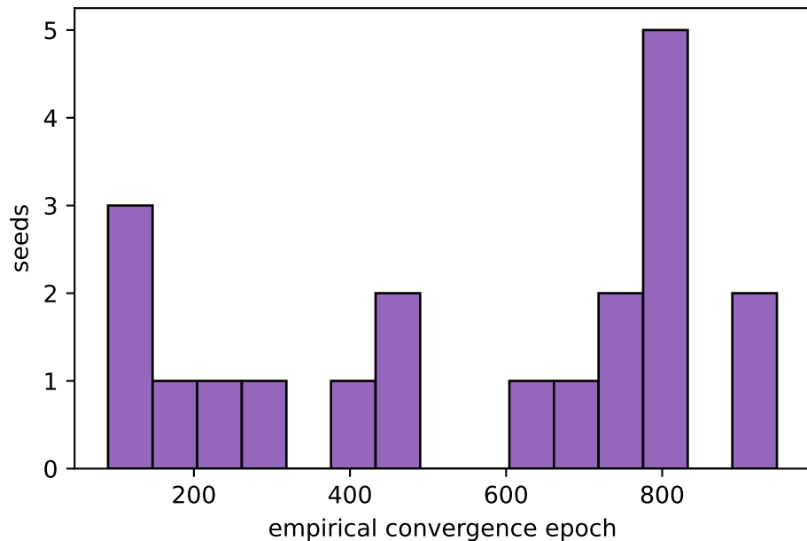
Empirical convergence epoch (mean=550, vs. \sim 50 at the original lr=0.05)
