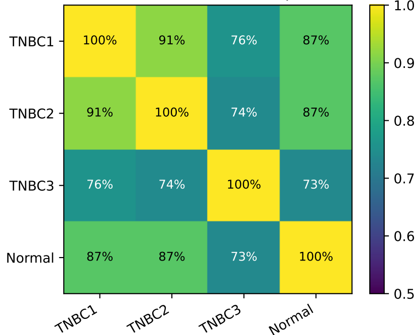
Compartment-sign agreement, chr18, all four real samples
