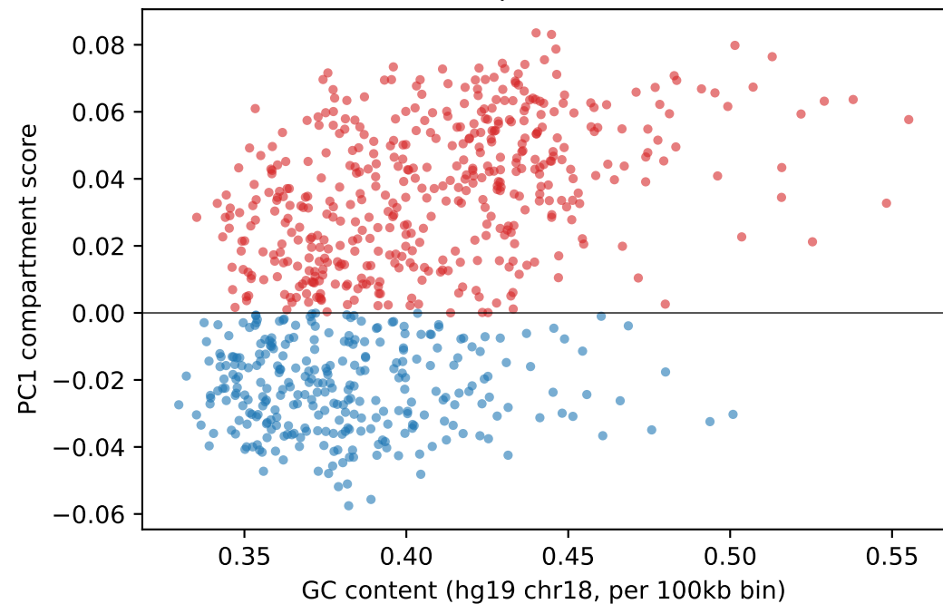
TNBC_Tissue3: PC1 vs. real GC content ( r=0.45 , independent validation)
