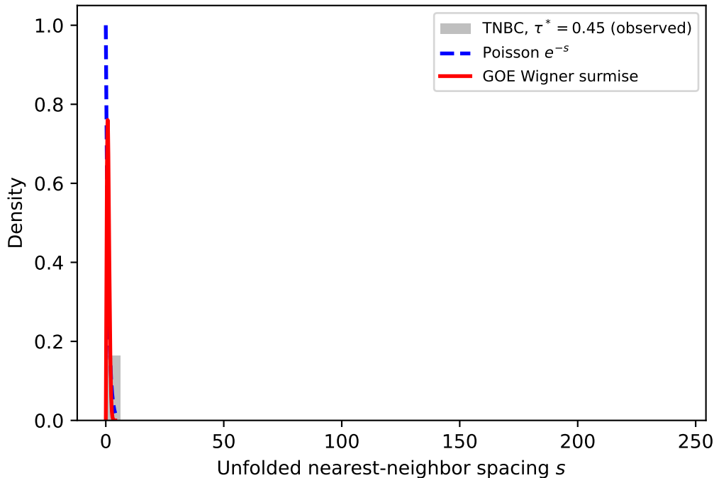
Level-spacing distribution at the RMT threshold (TNBC)
