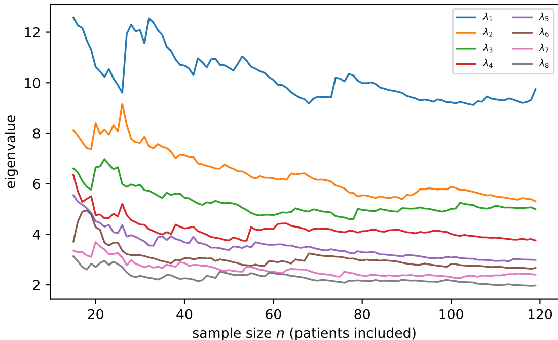
Top-8 eigenvalue trajectories, TNBC correlation matrix (fixed random patient-inclusion order)
