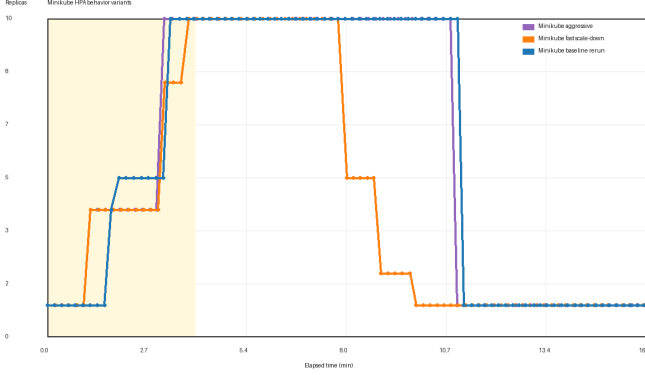
Fig. 3. Desired replicas in the Minikube behavior-tuning runs. All runs used the same 240 s active-load window and 720 s post-load observation window.
