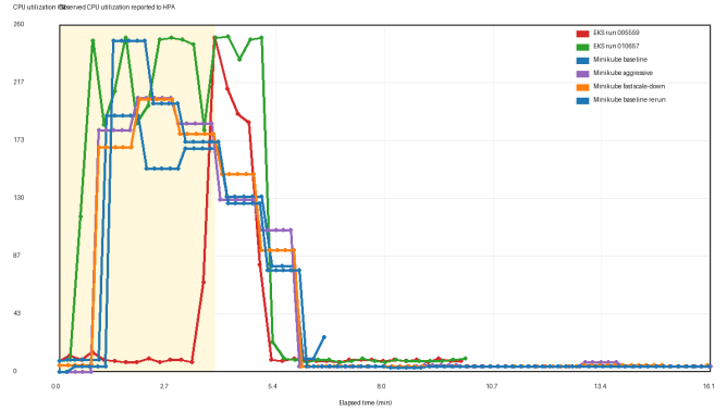
Fig. 4. CPU utilization reported to HPA. EKS remains above target while workload pods are pending, showing that the desired replica count alone did not provide enough effective capacity.
