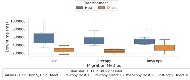
Figure B.90.: TCP Client downtime comparison under TEE Worst.
