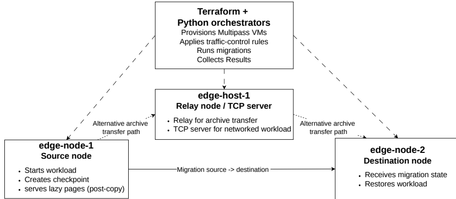
Figure 3.1.: Simplified test environment used by the benchmark framework.
