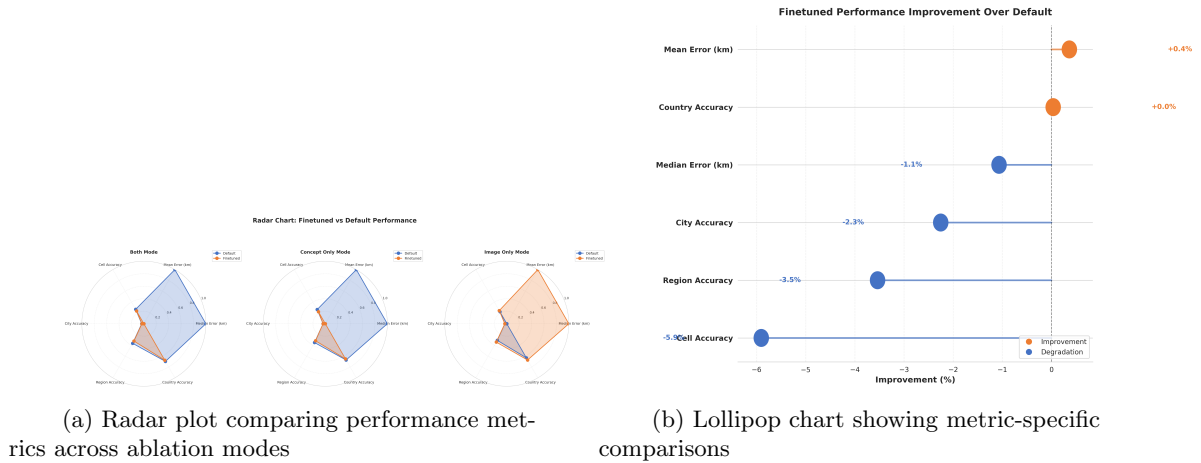
Figure 4: Ablation analysis for the finetuned model variant. The “both” mode (combining concepts and cross-attention) achieves the best overall performance, but concept-only predictions remain competitive, validating the interpretability of the concept bottleneck.
