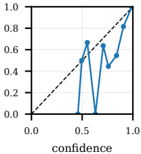
in_domain_test_temperature_scaled ECE=0.0109
