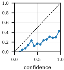
cross_domain_plantdoc_core_temperature_scaled ECE=0.3978
