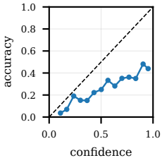
cross_domain_plantdoc_core ECE=0.2535
