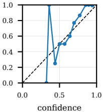
in_domain_test ECE=0.1095
