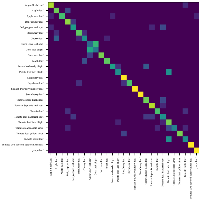
pdc_efficientnet_b0_s42 — in_domain_test (row-normalised)
