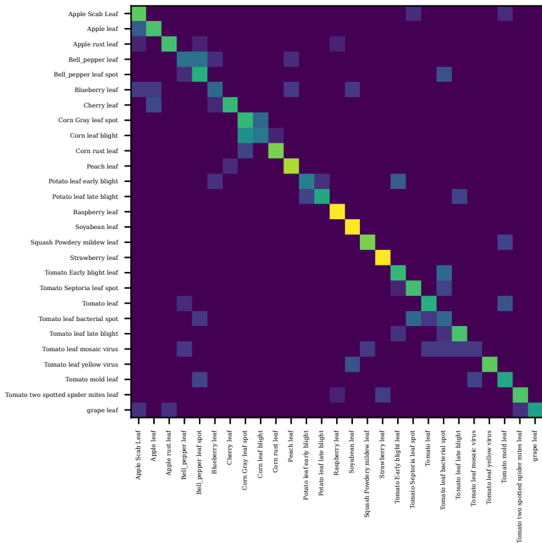
pdc_mobilenet_v3_small_s1337 — in_domain_test (row-normalised)
