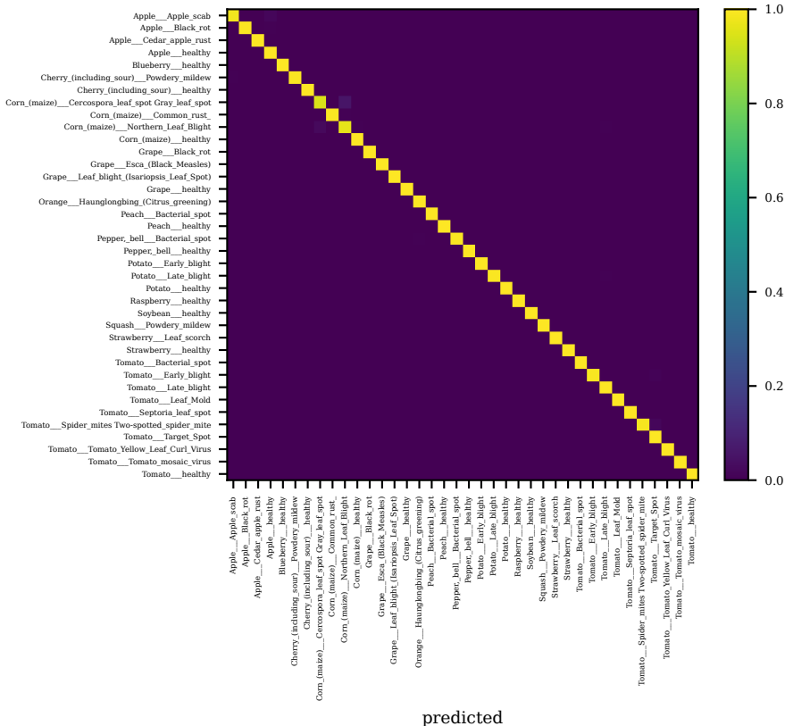
pv_efficientnet_b0_s42 — in_domain_test (row-normalised)
