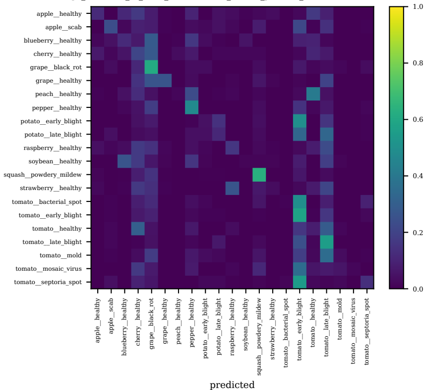
pv_mobilenet_v3_small_s1337 — cross_domain_plantdoc_core (row-normalised)
