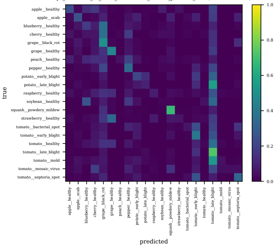
pv mobilenet v3 small s42 — cross domain plantdoc core (row-normalised)
