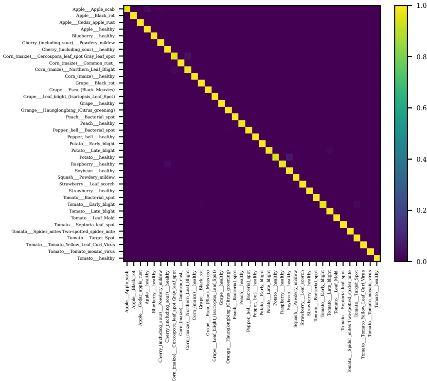
pv_mobilenet_v3_small_s42 — in_domain_test (row-normalised)
