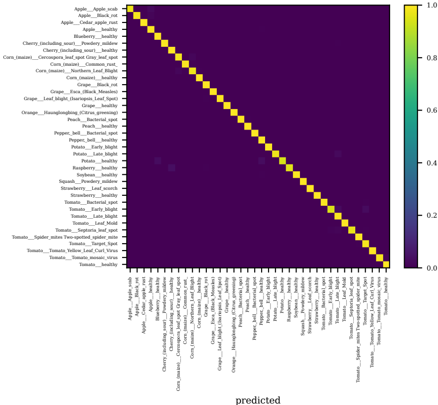
pv_resnet50_s42 — in_domain_test (row-normalised)
