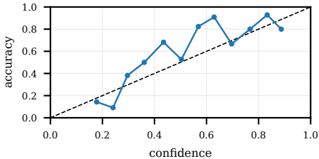
in_domain_test ECE=0.1345
