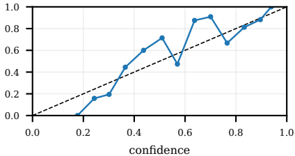
in_domain_test_temperature_scaled ECE=0.1182
