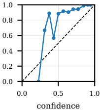
in_domain_test ECE=0.1013
