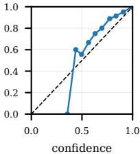
in_domain_test_temperature_scaled ECE=0.0095
