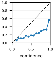
cross_domain_plantdoc_core_temperature_scaled ECE=0.2790
