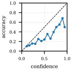
cross_domain_plantdoc_core ECE=0.1356
