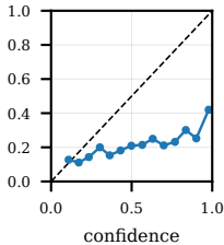
cross_domain_plantdoc_core ECE=0.4305
