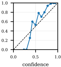
in_domain_test ECE=0.0903
