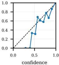
in_domain_test_temperature_scaled ECE=0.0094
