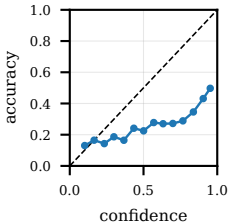
cross_domain_plantdoc_core ECE=0.3038
