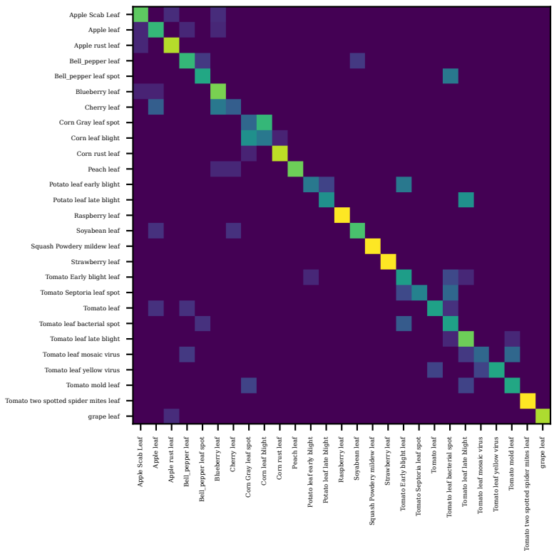
pdn_resnet50_s2026 — in_domain_test (row-normalised)
