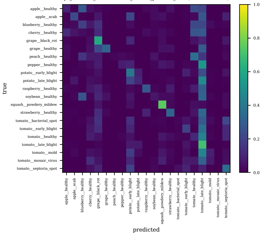
pv_resnet50_s2026 — cross_domain_plantdoc_core (row-normalised)
